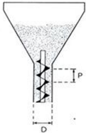
Gambar 6.8 Volumetric Auger Filler (paine dan Paine, 1993).
