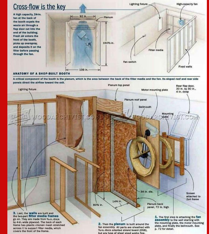
•Spray Booth
