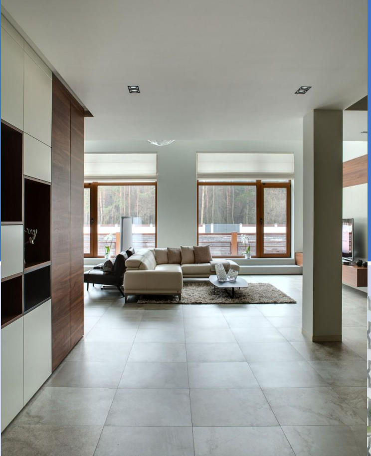
PARALLEL PLANES
